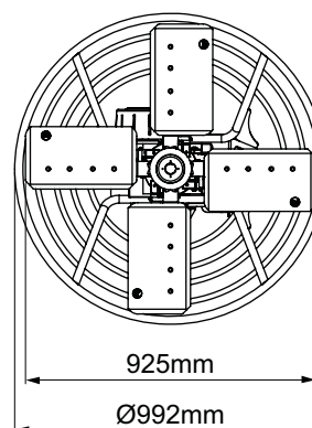
TROWELLING DIAMETER & RING DIAMETER
